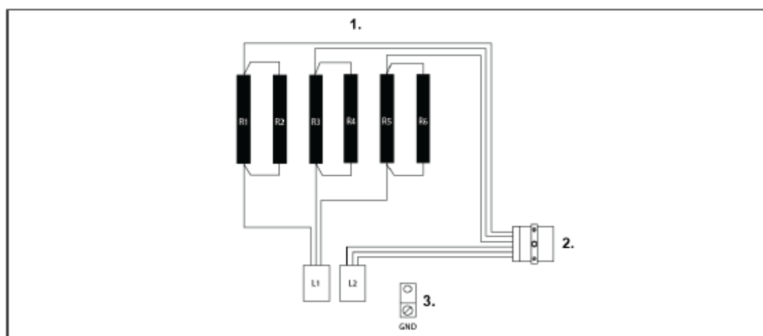
Wiring diagram
